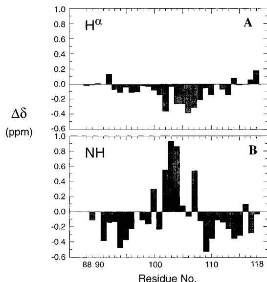
FIGURE 8: Difference between the chemical shift of a given resonance in 30% v/v TFE and the shift in 90% 1 H 2 O/10% 2 H 2 O plotted against residue number for (A) C α H and (B) NH resonances.
